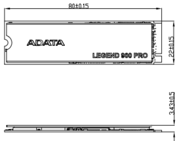
<With heatsink>
