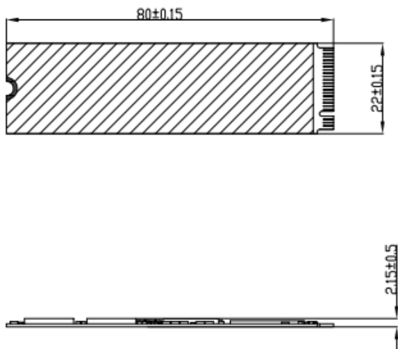
<Without heatsink>
