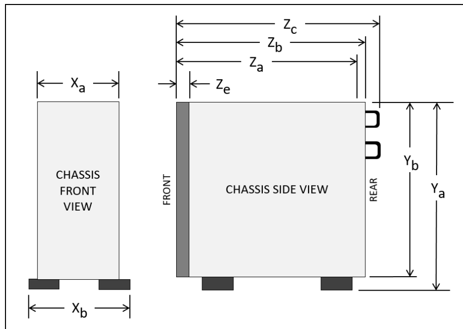
Figure 14. Server dimension
