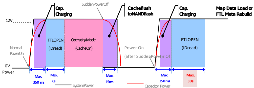
Figure 2. Sudden Power on-off operation
