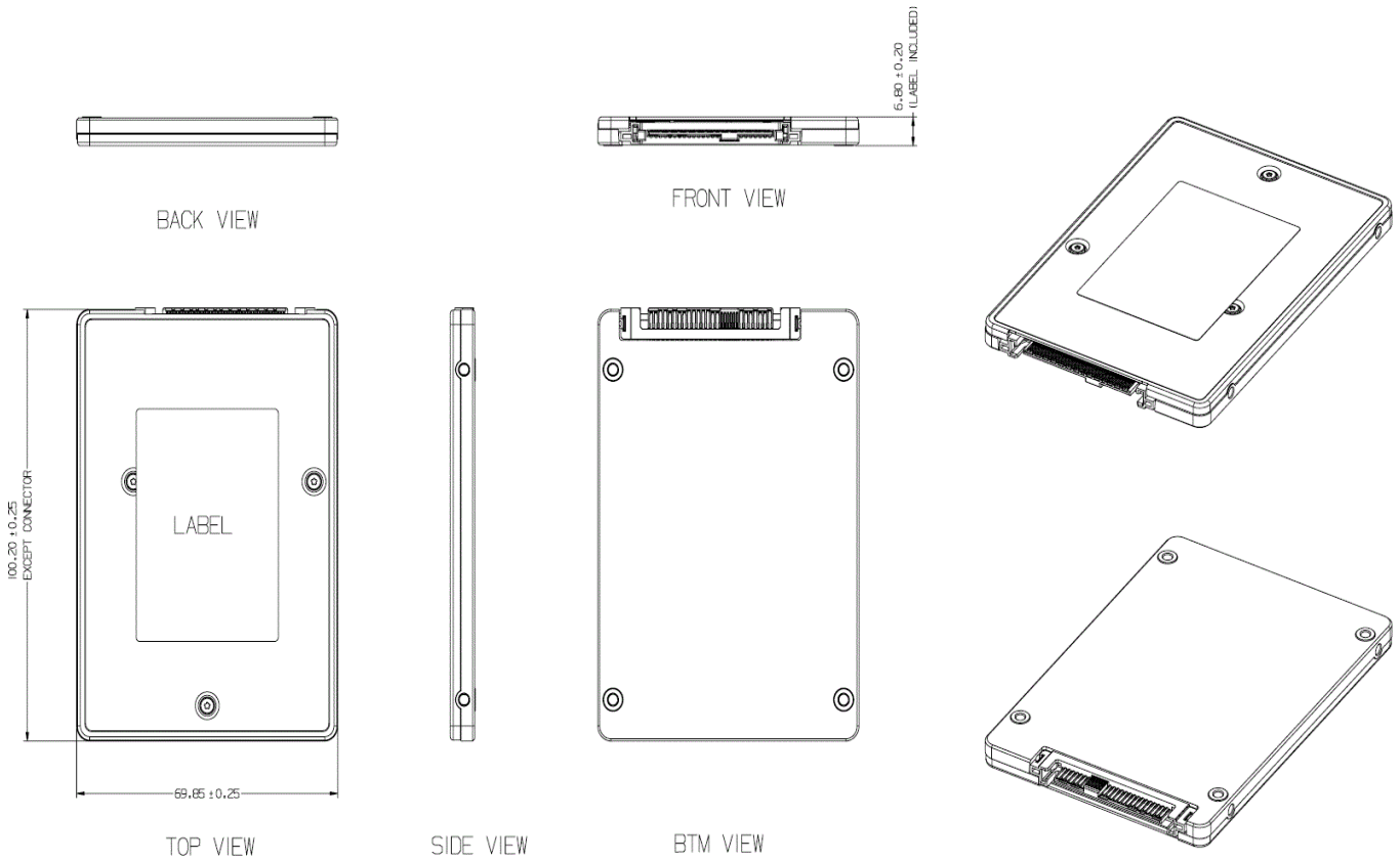
Figure 1. Mechanical Outline
